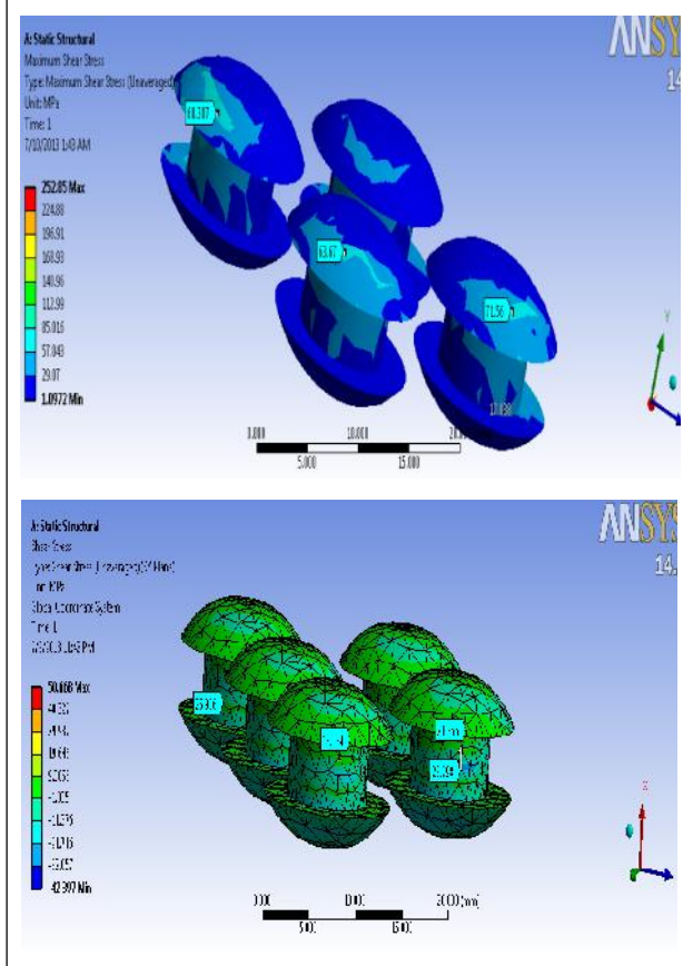
Figure 9: Maximum Shear Stress on Rivet
