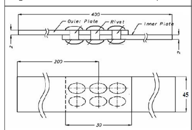
Figure 4: Geometric of Riveted Lap Joint
