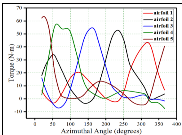
Figure 9. Predicted Torque generated by each airfoil at 10m/s with 28 rad/s
