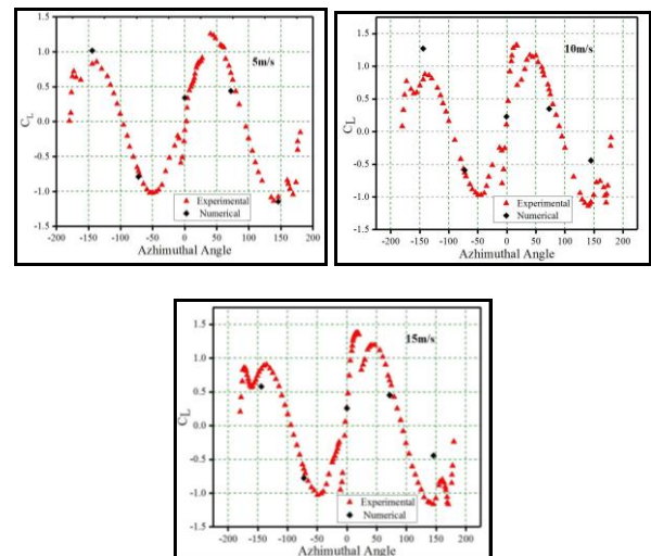
Figure 4. Comparison of experimental and numerical static analysis lift plot on each airfoil at different azimuthal angle.
