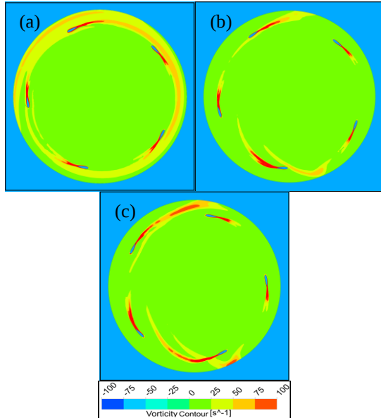
Figure 8. Predicted Vorticity field for the five bladed rotor computed using Realizable k- \epsilon model with (a) 12rad/s at 5m/s, (b) 24rad/s at 10 m/s and (c) 36 rad/s at 15m/s
