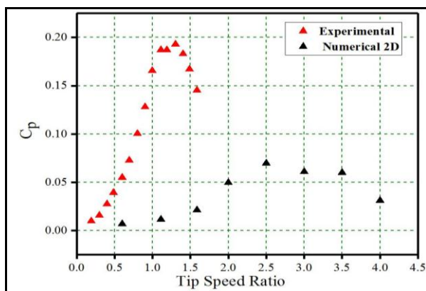
Figure 5. Performance curve of three bladed H-Darrieus turbine versus TSR with experimental data.
