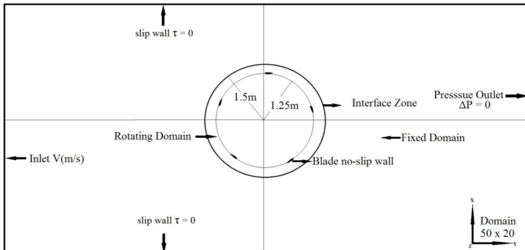
Figure 1. Computational wind tunnel domain dimensions and boundary conditions.
