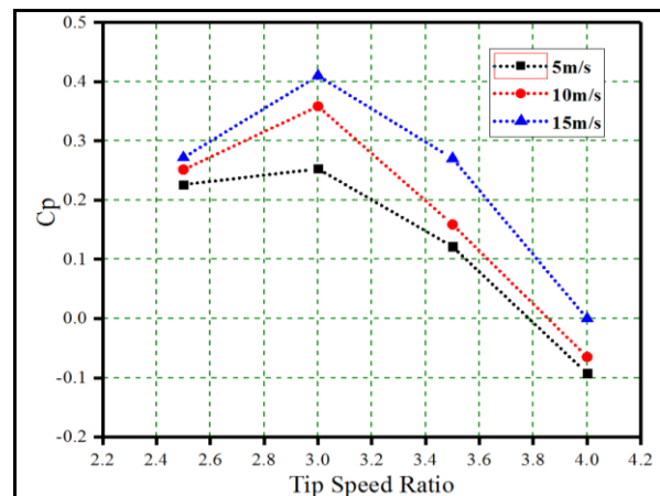
Figure 7. Performance curve of five bladed H-Darrieus turbine versus TSR with experimental data.
