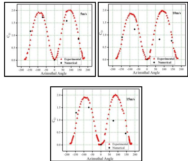
Figure 3. Comparison of experimental and numerical static analysis drag plot on each airfoil at different azimuthal angle.
