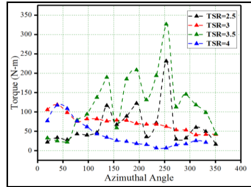
Figure 10. Predicted Torque versus Tip at speed ratio at 10 m/s
