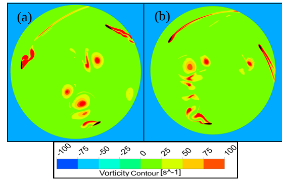
Figure 6. Predicted Vorticity field for the three bladed rotor computed using Realizable k- \epsilon model with (a) 9.6 rad/s and (b) 12.8 rad/s with a velocity 8 m/s.
