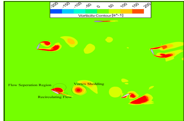
Figure 2. Predicted vorticity field for static analysis at 15m/s.
