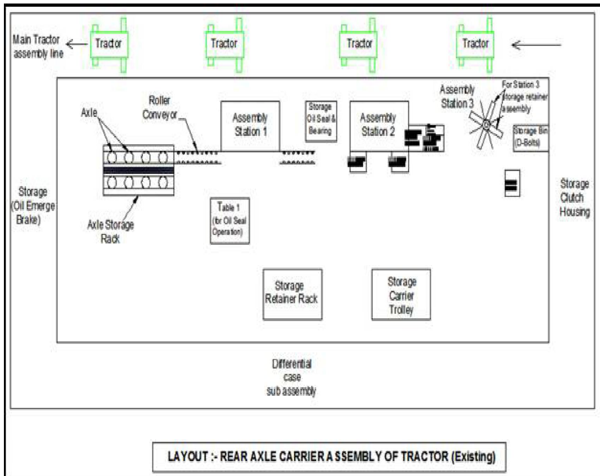
Figure 1: Rear Axle Carrier Assembly of Tractor (Existing)
