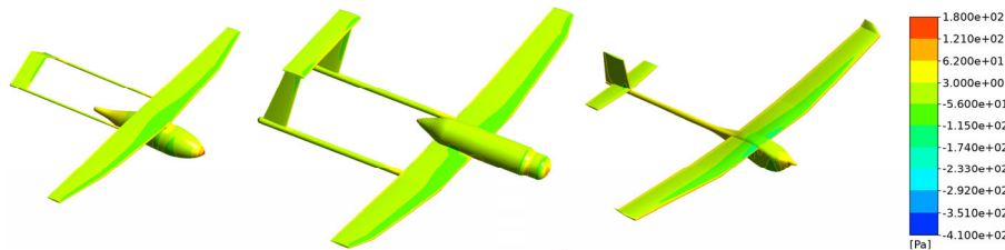
Fig. 6. Surface pressure contours of UAV 2, UAV 3, and UAV 9 with a common pressure legend (Cruise speed: 17 m/s).
