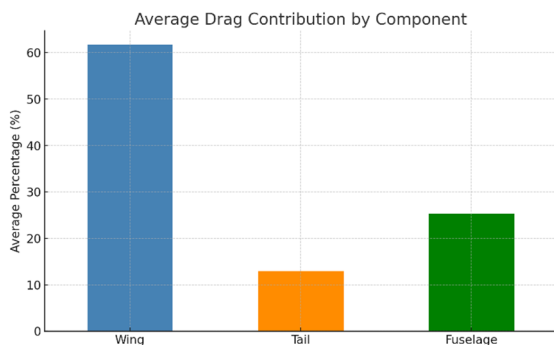
Fig. 9. Component drag distribution.
