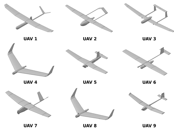
Fig. 1. Reconstructed OpenVSP models of the nine representative mini electric UAV configuration.
