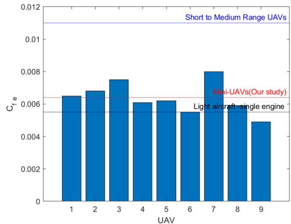
Fig. 10. The equivalent skin friction coefficient for Small/Mini UAVs.
