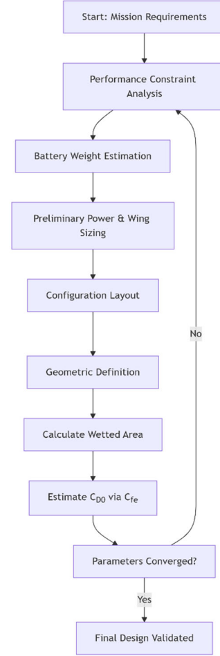
Fig. 4. Diagram process of conceptual design.
