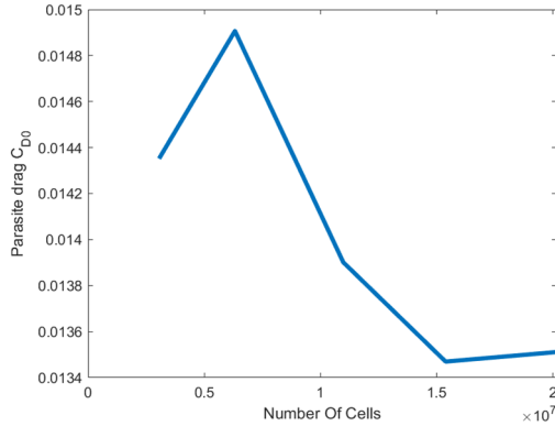
Fig. 3. Mesh convergence study for UAV8.
