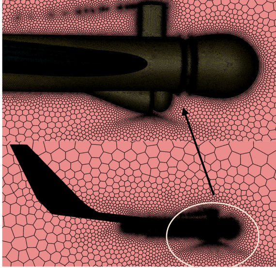
Fig. 2. Mesh discretization and boundary layer for UAV8.
