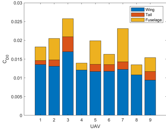
Fig. 8. Drag coefficient for with components distribution different UAVs.
