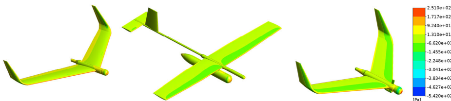
Fig. 7. Surface pressure contours of UAV 4, UAV 6, and UAV 8 with a common pressure legend (Cruise speed: 20 m/s).
