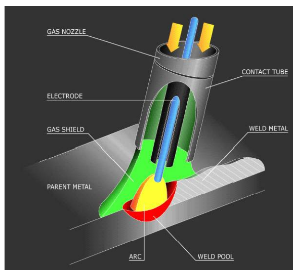
Figure 1: Working Principles of GMAW
