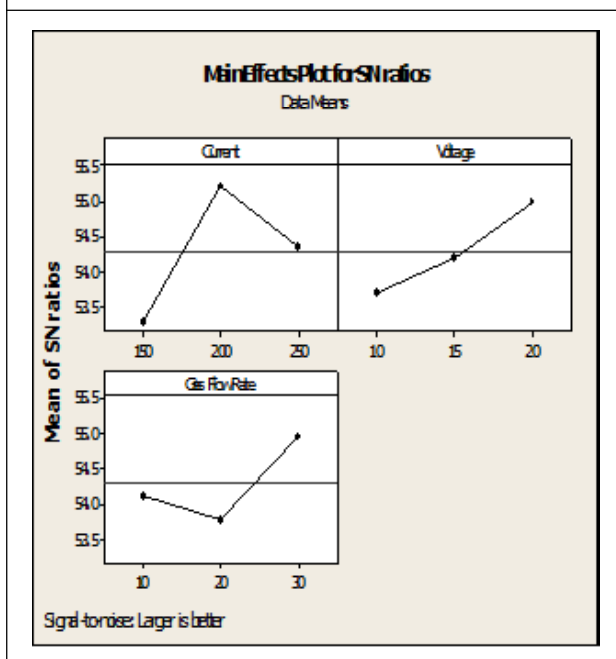
Figure 3: Main Effects Plot for S/N Ratio-Tensile Strength
