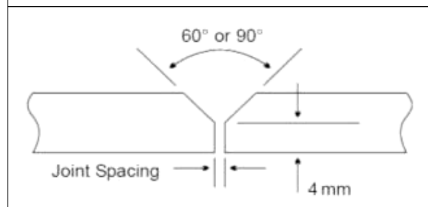
Figure 2: Joint Geometry for the Welding Specimens
