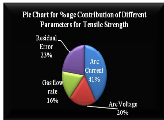
Figure 4: Pie Chart for %age Contribution of Different Parameters for Tensile Strength
