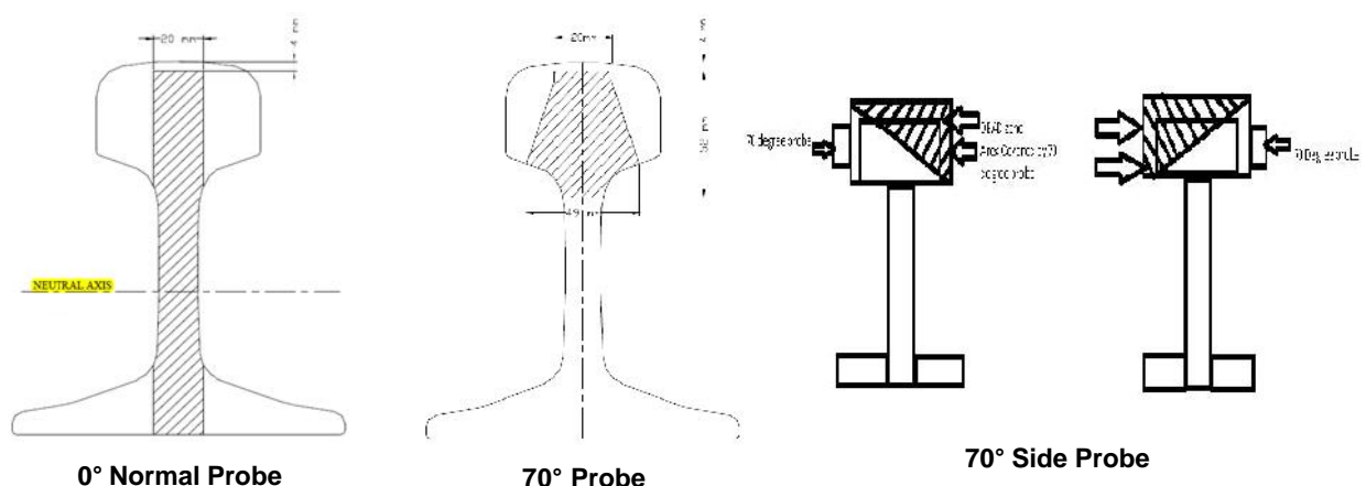
Figure 10: Different Types of Probes
