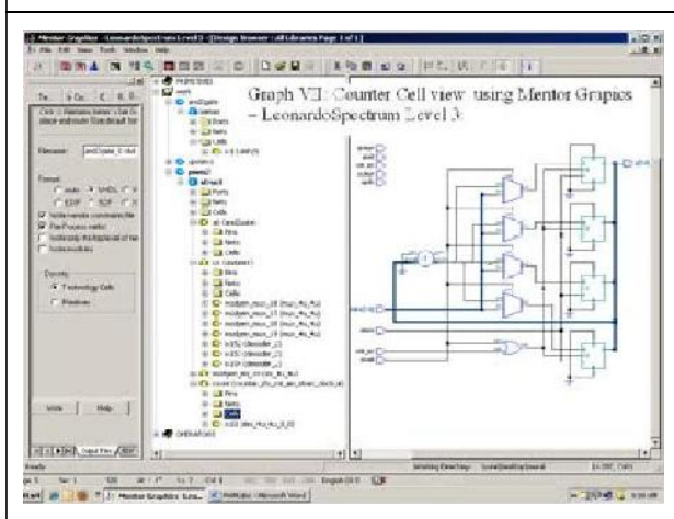
Graph 7: Counter Cell View Details Using Mentor Graphics – Leonardo Spectrum RTL Schematic
