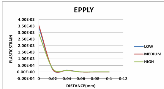
Figure 18: Effect of heat Input on Plastic Strain Along Y Direction
