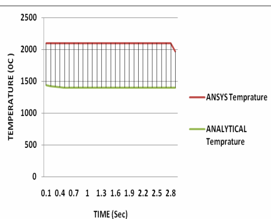
Figure 35: Comparison Between Analytical and ANSYS Temperature
