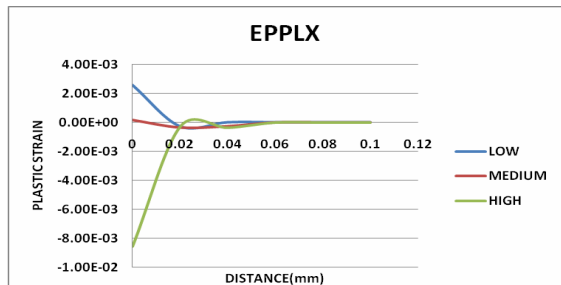
Figure 29: Effect of Speed on Plastic Strain Along X Direction
