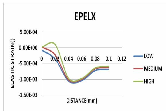
Figure 14: Effect of Heat Input on Elastic Strain Along X Direction
