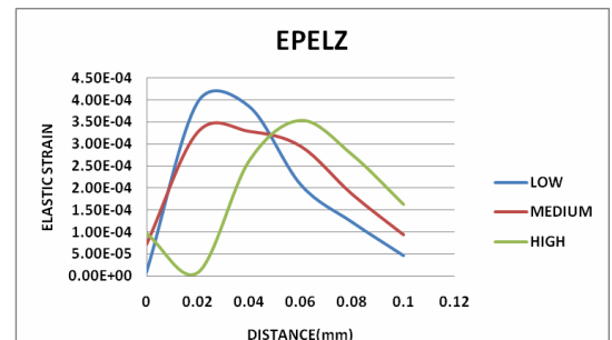
Figure 28: Effect of Speed on Elastic Strain Along Z Direction
