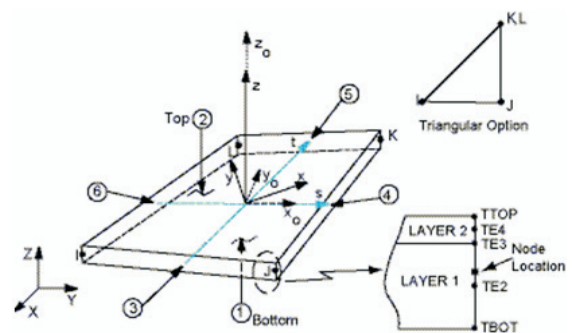
Figure 7: Geometry of Shell 131 Element
