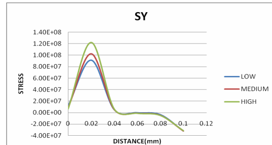
Figure 21: Effect of Heat Input on Stress Along Y Direction
