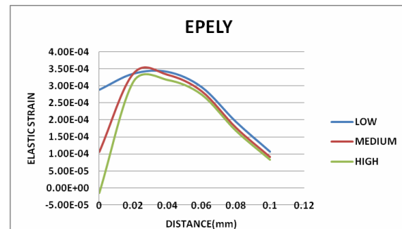
Figure 15: Effect of Heat Input on Elastic Strain Along Y Direction
