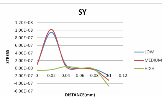
Figure 33: Effect of Speed on Stress Along Y Direction
