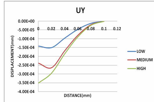
Figure 24: Effect of Speed on Displacement Along Y Direction
