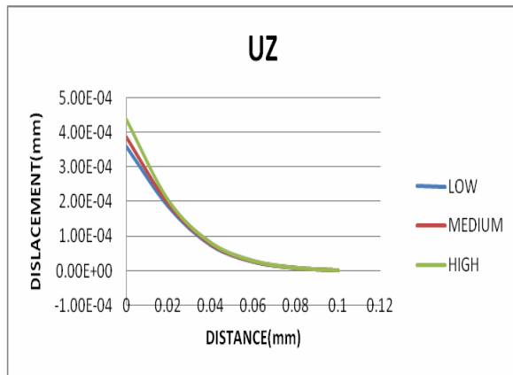
Figure 13: Effect of Heat Input on Displacement Along Z Direction
