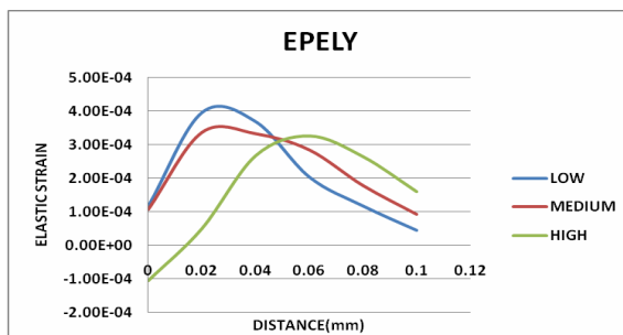
Figure 27: Effect of Speed on Elastic Strain Along Y Direction
