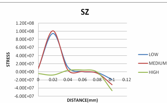
Figure 34: Effect of Speed on Stress Along Z Direction
