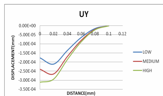
Figure 12: Effect of Heat Input on Displacement Along Y Direction
