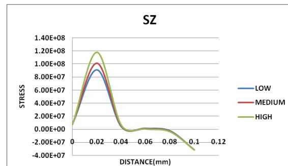
Figure 22: Effect of Heat Input on Stress Along Z Direction
