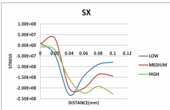
Figure 32: Effect of Speed on Stress Along X Direction
