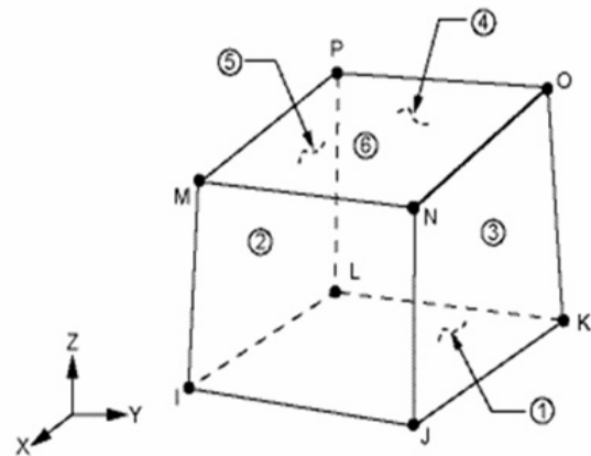
Figure 6: Geometry of Solid 70 Element
