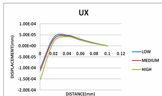
Figure 11: Effect of Heat Input on Displacement Along X Direction
