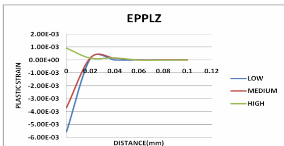
Figure 31: Effect of Speed on Plastic Strain Along Z Direction
