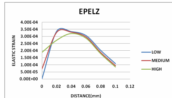
Figure 16: Effect of Heat Input on Elastic Strain Along Z Direction
