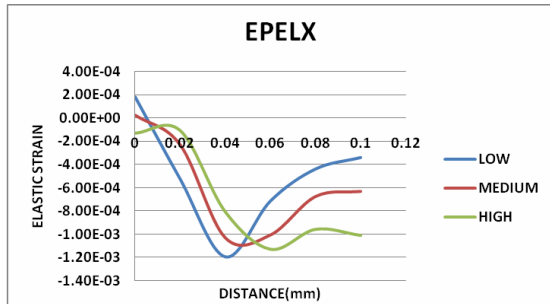
Figure 26: Effect of Speed on Elastic Strain Along X Direction
