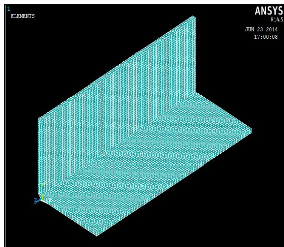
Figure 8: Meshing of the Welded Plates
