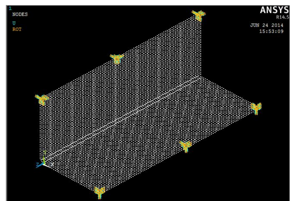
Figure 10: Boundary Condition Applied to the Structural Welded Plates
