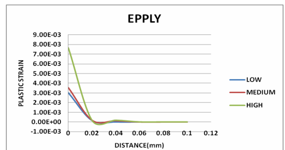
Figure 30: Effect of Speed on Plastic Strain Along Y Direction
