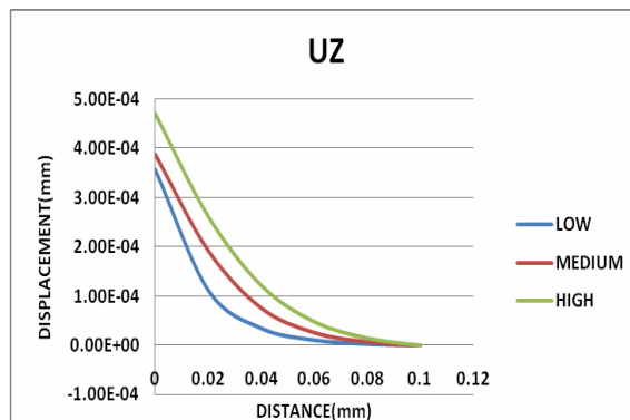
Figure 25: Effect of Speed on Displacement Along Z Direction
