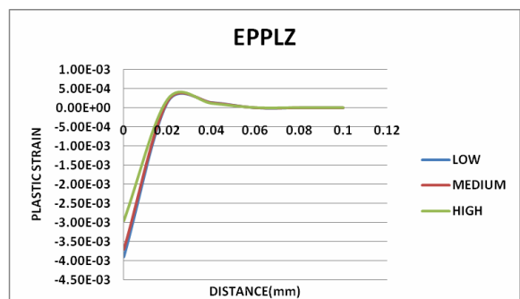
Figure 19: Effect of Heat Input on Plastic Strain Along Z Direction
