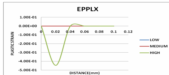
Figure 17: Effect of Heat Input on Plastic Strain Along X Direction
