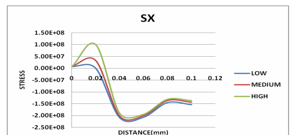
Figure 20: Effect of Heat Input on Stress Along X Direction
