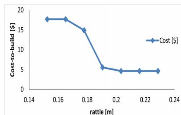
Figure 4: A Single 2D Plane from the 5D Pareto Optimal Set Showing the Trade-Off Between the Cost-to-Build Objective and Rattle Constraint Bound; the Other Constraints are Held Constant at \bar{J}_{ride} = 220[m^2/s^3] , and \bar{J}_{holding} = 0.03[m]
