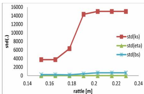
Figure 6: Optimally Apportioned Uncertainties Determined from the New Simultaneous OUA/RDO Framework. The First Two Points were Infeasible Designs and Therefore the Values were Set to their Initial Values
