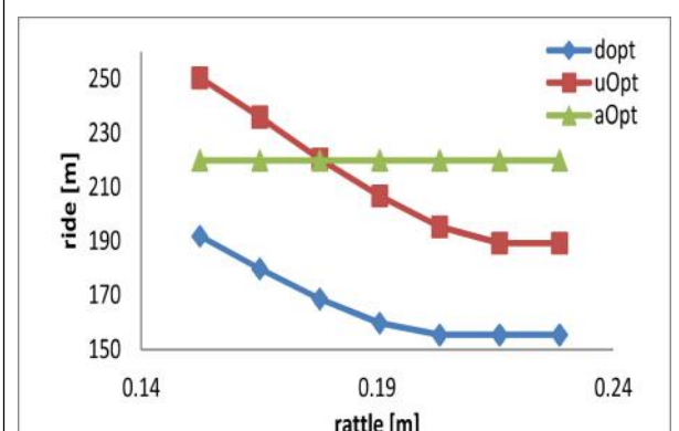
Figure 5: A Single 2D Plane Showing the Trade-Off Between the Ride Objective and Rattle Constraint Bound When Performing an RDO Design; where \bar{J}_{holding} = 0.034[m] is Held Fixed. The Triangle Curve Represents the Bounding Value for \bar{J}_{ride} When Performing the OUA/RDO Designs Associated with Figure 3 and Figure 4. The First Two Points on the Triangle Curve Require Too Large of a Reduction in Uncertainties and Therefore Result in Infeasible aOpt Designs
