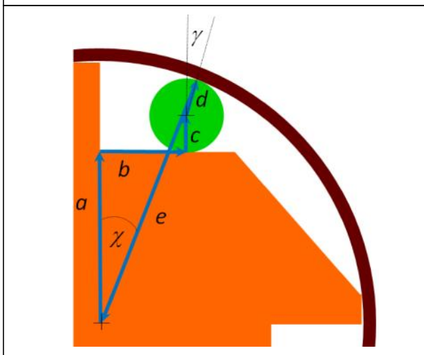
Figure 1: One Quarter of a Clutch Assembly. The Independent Variables are Dimensions \{a, c, d, e\} and the Dependent Variables are \{b, t, x\} . Proper Operation of the Clutch Requires 6^\circ \leq t \leq 8^\circ
