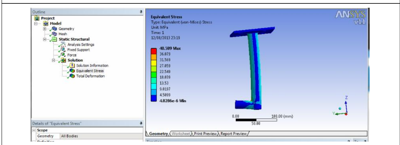
Figure 8: Equivalent Stress
