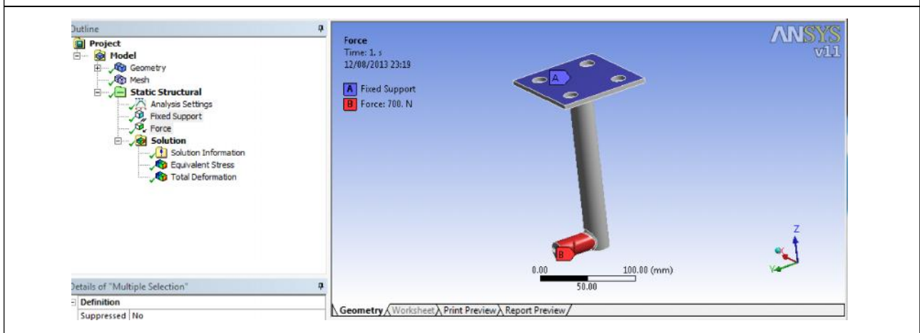
Figure 7: Loading Conditions
