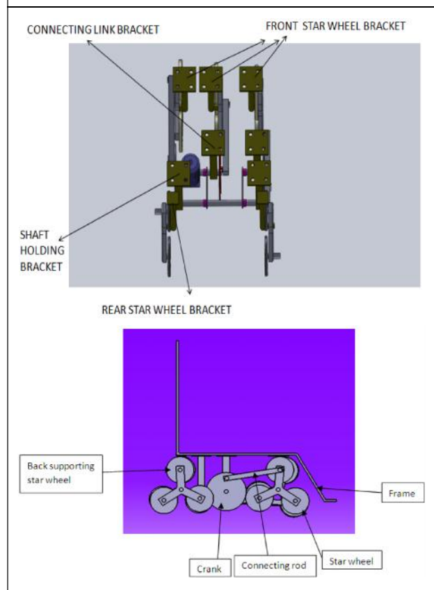
Figure 4: Complete Mechanism of Stair Climbing Chair
