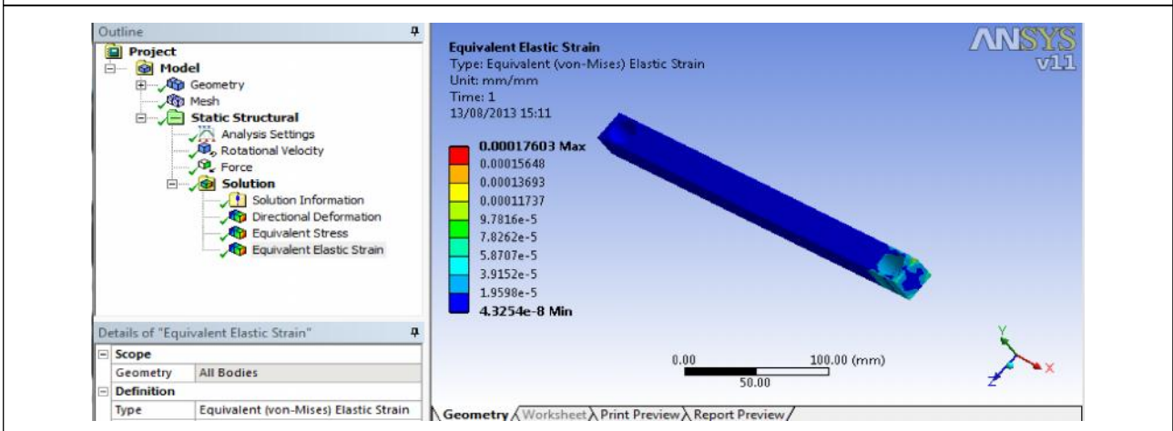
Figure 13: Equivalent Elastic Strain
