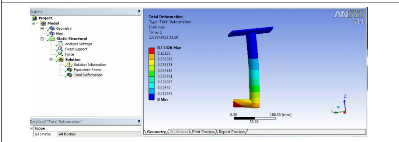
Figure 9: Deformation
