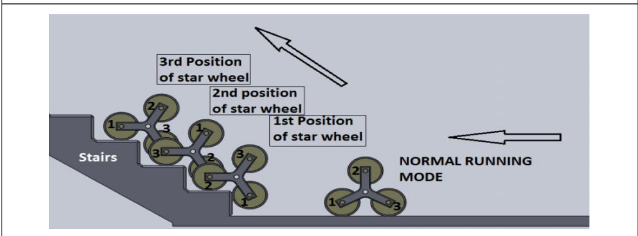
Figure 14: Simulation Result
