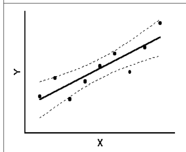
Figure 3: Prediction Intervals
