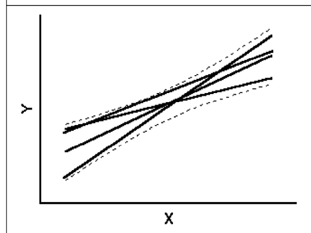
Figure 4: Confidence Graph
