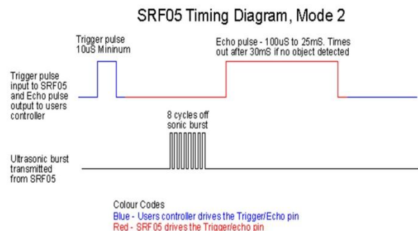
Figure 6. Timing diagram, mode 2
