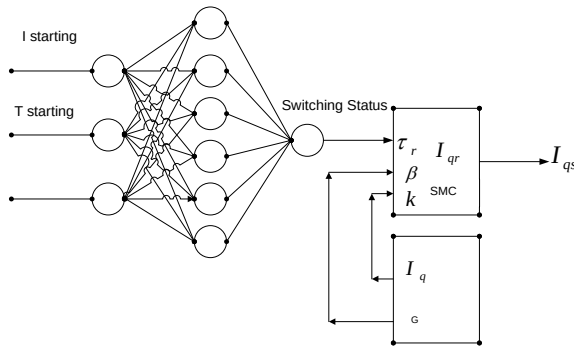
Figure 8. Model diagram of artificial neural network with sliding mode control
