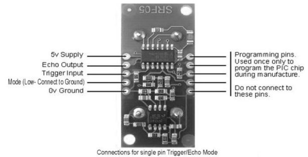
Figure 5. Single-pin SRF ultrasonic
