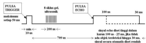
Figure 12. SRF 05 MODE 2 timing Diagram
