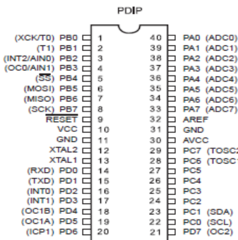
Figure 10. Pin out ATMEGA 8535
