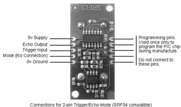
Figure 3. Compatible ultrasonic type
