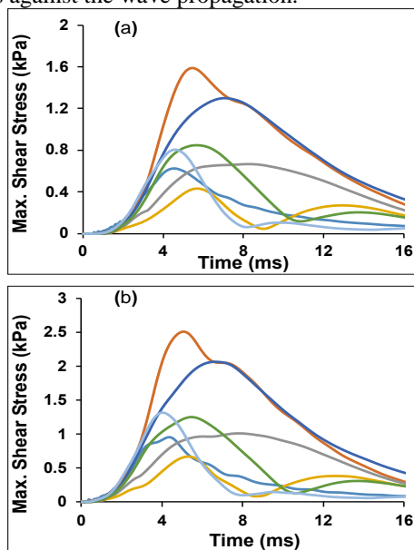
Figure 5. Maximum shear stress responses of the NDSUFEHM for (a) low-velocity impact; (b) High-velocity impact
