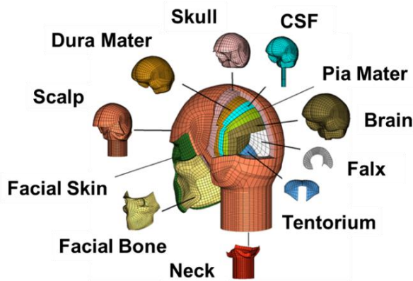
Figure 2. FE discretization of human head components for NDSUFEHM.
