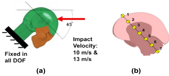
Figure 3. (a) Boundary conditions and head orientation at 45 °from Frankfurt plane; (b) sagittal plane of the brain and the schematic view of the locations that the biomechanical parameters are extracted.
