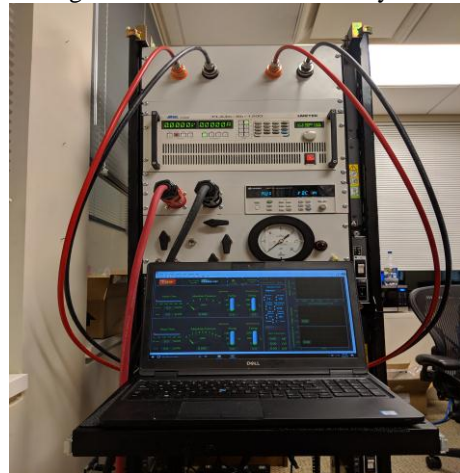
Figure 5. Test stand designed and integrated in-house for testing fuel cells up to 4 kW electrical power.
