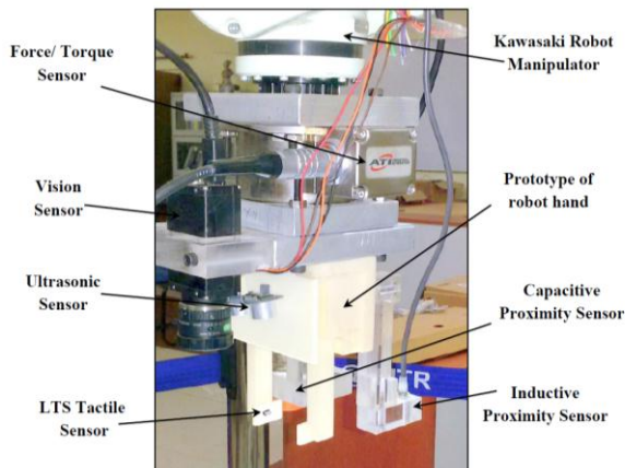
Figure 6. Sensors integrated robotic hand.
