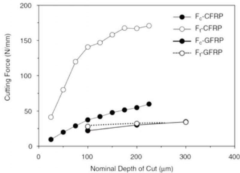
Figure 5: Relationship Between Nominal Depth of Cut and Cutting Forces in Machining CFRP and GFRP. Fibre Orientation \theta = 30^\circ , Nose Radius = 50 \mu\text{m}
