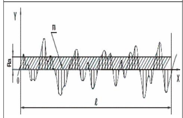
Figure 6: Measurement of R_a
