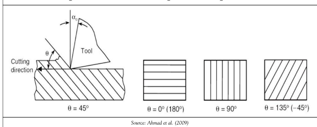
Figure 2: Fibre Orientation Angle w.r.t Cutting Direction
