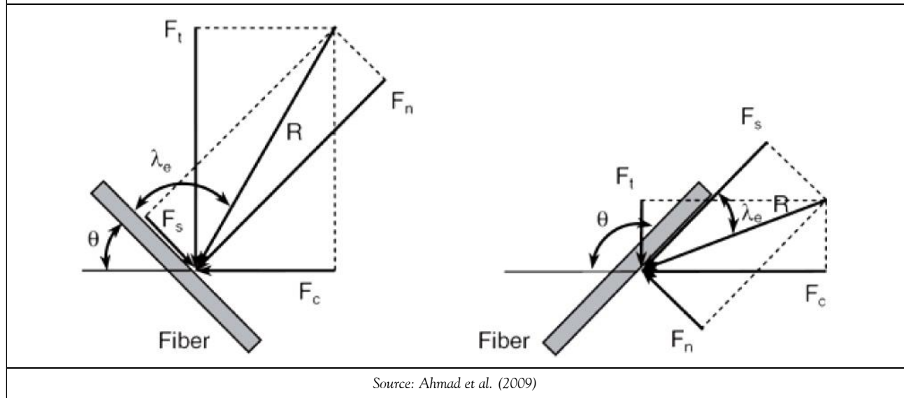
Figure 3: Force Components Along and Perpendicular to the Plane of the Fibres
