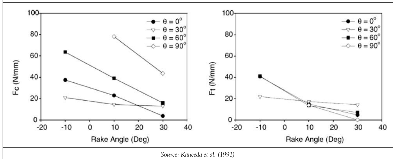
Figure 4: Cutting Force vs. Rake Angle and Vertical Force vs. Rake Angle When Cutting CFRP. v = 0.02 m/min, a_c = 0.1 mm and a_w = 2.28 mm
