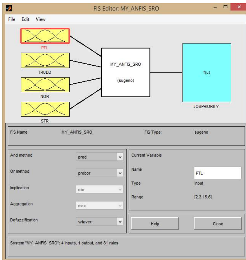
Figure 4: Developed SANFIS (MY_ANFIS_SRO.FIS) Layout
