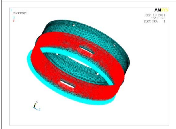
Figure 9: Harmonic Load for Zone 3 Turning
