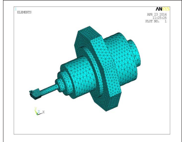
Figure 3: Finite Element Meshed Model of the High Speed Spindle Unit
