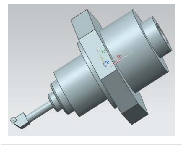
Figure 2: Isometric view of the spindle and tool assembly
