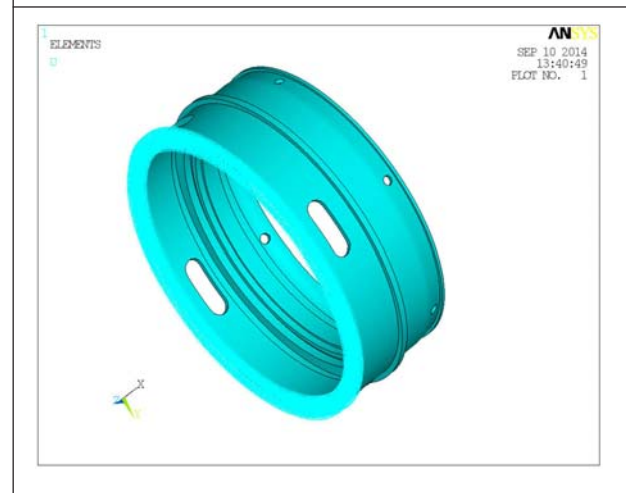
Figure 6: Boundary Conditions for Modal Analysis
