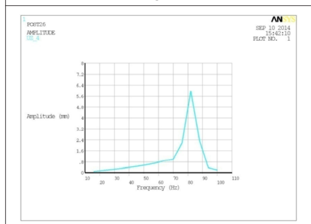
Figure 12: Frequency Vs Amplitude in Z-dir Graph for Zone3
