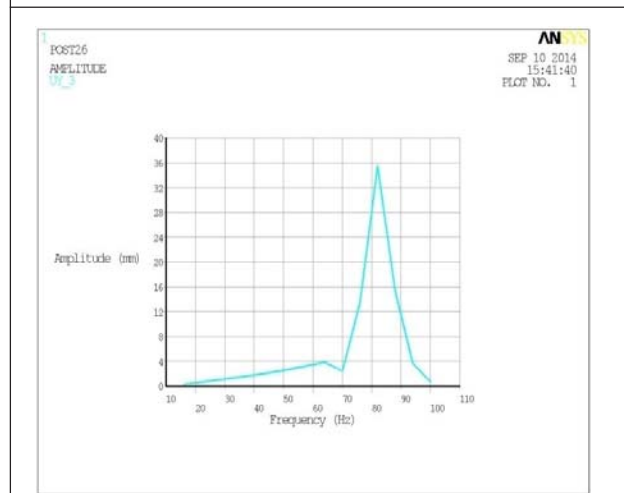
Figure 11: Frequency Vs Amplitude in Y-dir Graph for Zone3
