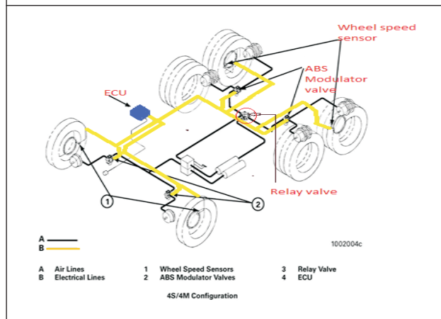
Figure 4: 4S/4M Configuration
