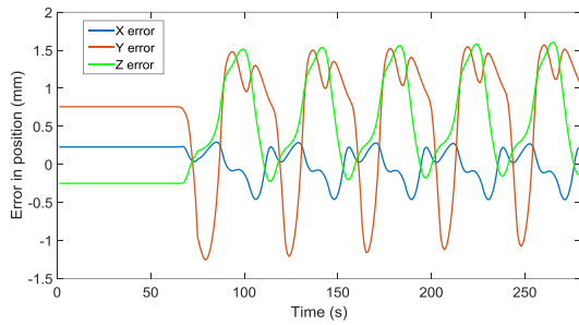
Figure 14. ANN motion error in x, y, and z direction
