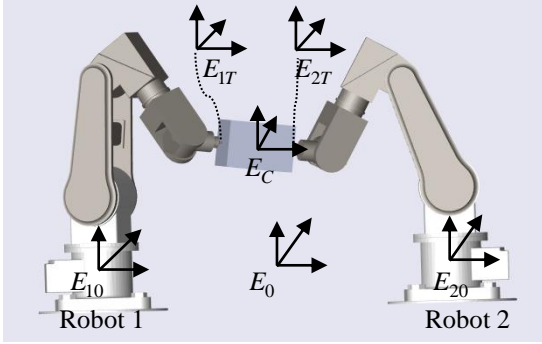
Figure 4. Cooperating robot arms carrying a rigid object.
