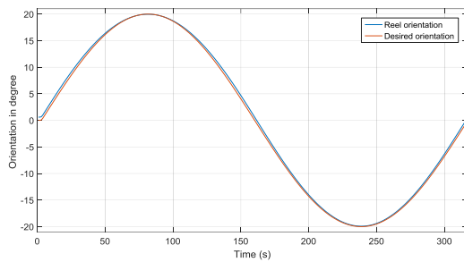
Figure 18. The comparison results of the desired and the actual orientation around the Y axis of the common object using ANN.
